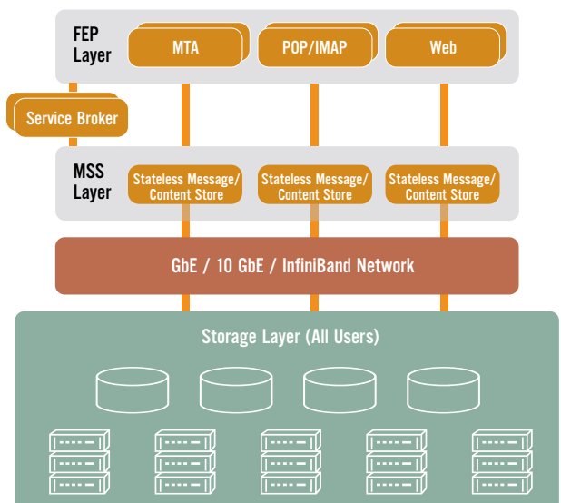
Figure 1: Openwave Stateless Message Store Architecture.
